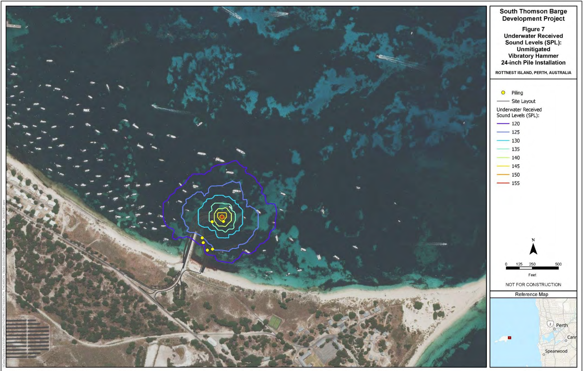
Figure 7. Underwater Received Sound Levels (SPL): Unmitigated Vibratory 24-inch Pile Installation
